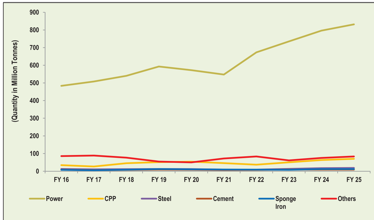
Chart 10: Year Wise Despatch of Coal to Different Priority Sectors from FY 2015-16 to FY 2024-25
