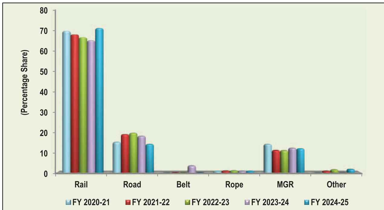
Chart 13: SCCL's Mode Wise Despatch of Coal during Last Five Years
